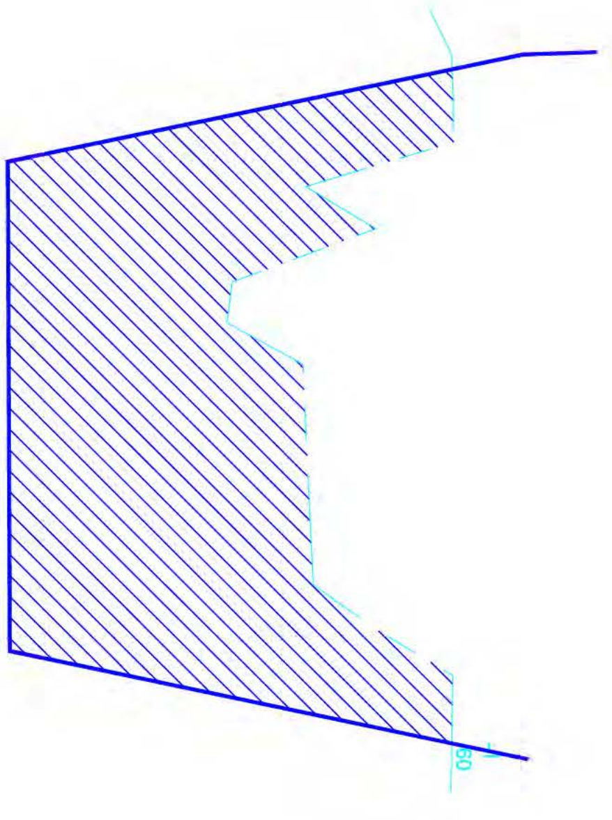
Cut Section, Sta. 0+60 0.32 cy/ft, 9.5 cy
